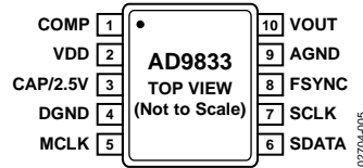
Figure 5. Pin Configuration
