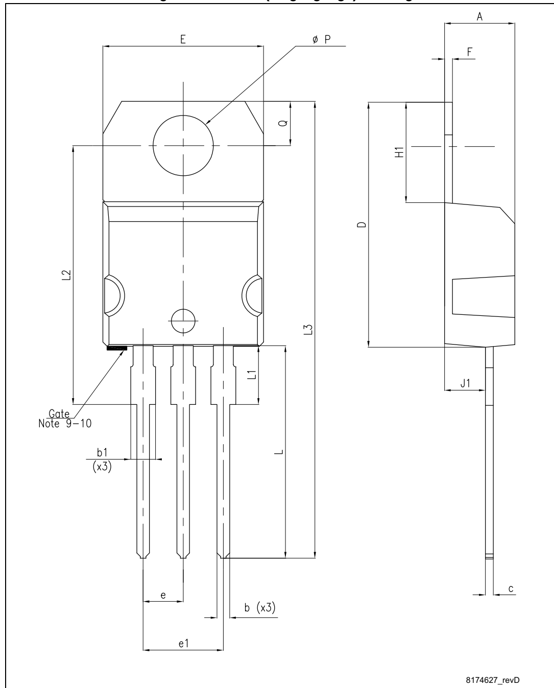
Figure 14. TO-220 (single gauge) drawing
